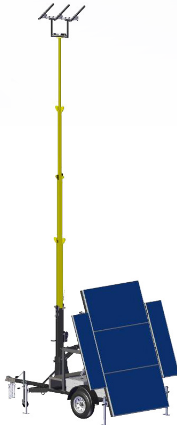
CT6 30' Mast
